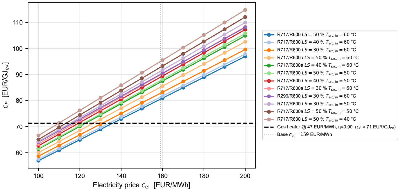
C_P vs electricity price — 12 cheapest designs ( T_{\text{steam}} = 120\text{ °C} )
