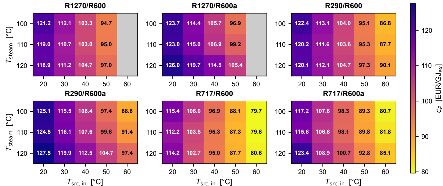
C_p heatmap over (T_{\text{src,in}}, T_{\text{steam}}) — best LS per cell
