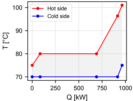
Internal HX (cycle-1 cond. / cycle-2 evap.)
