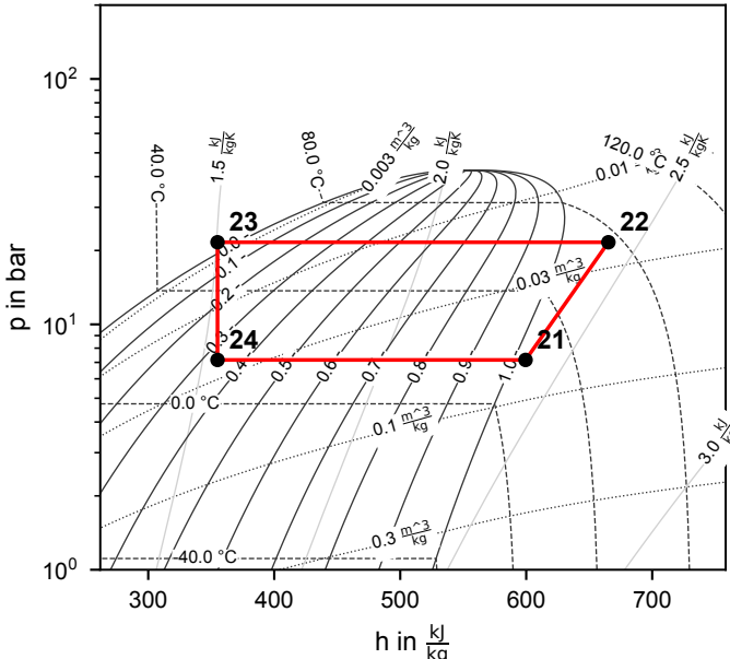
Cycle 1 (R290)
