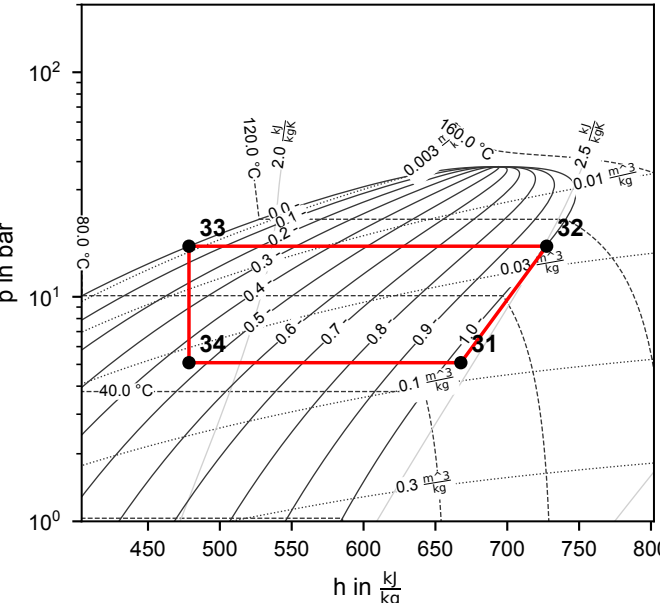
Cycle 2 (R600)
