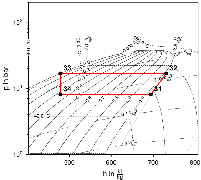
Cycle 2 (R600)
