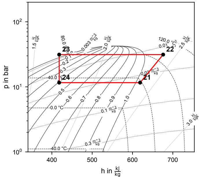
Cycle 1 (R290)
