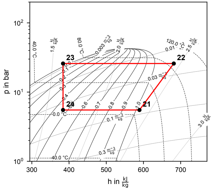
Cycle 1 (R290)
