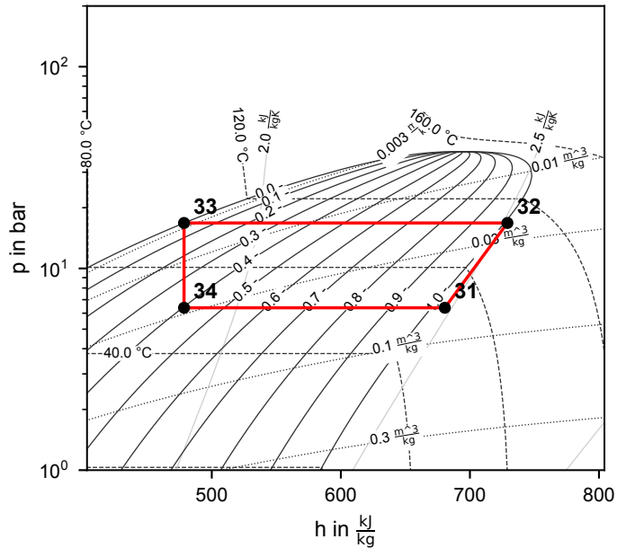
Cycle 2 (R600)
