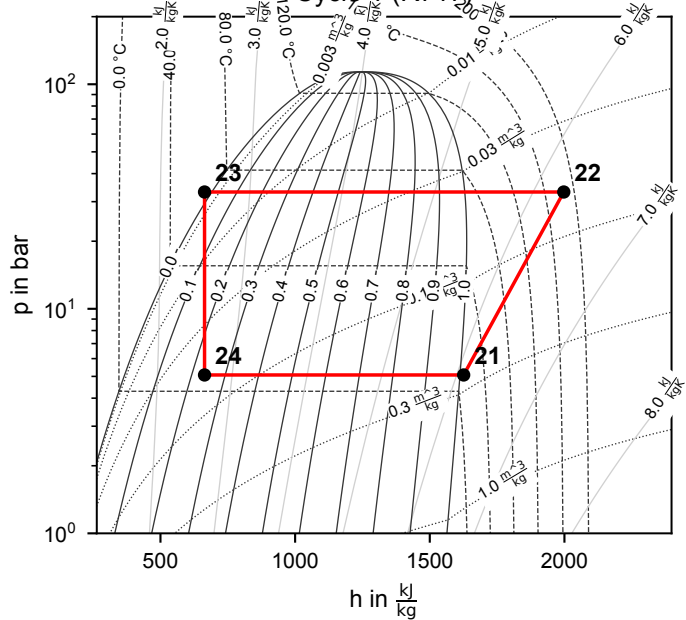
Cycle 1 (R717)
