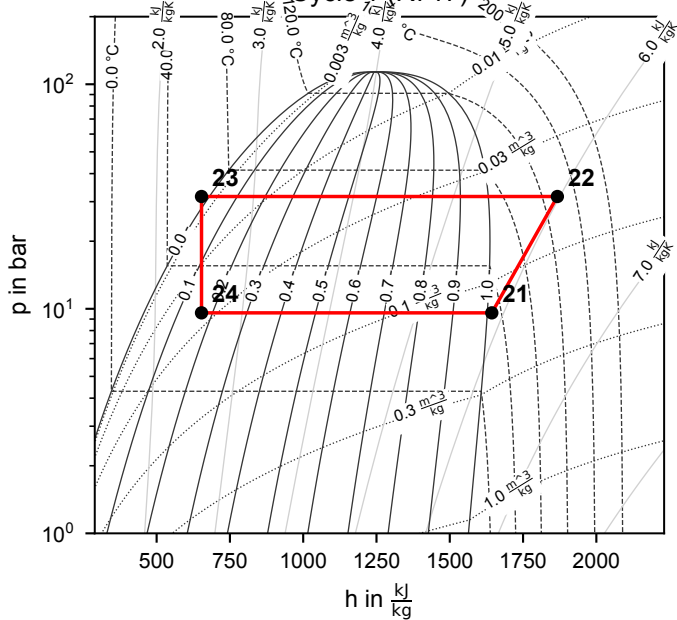
Cycle 1 (R717)
