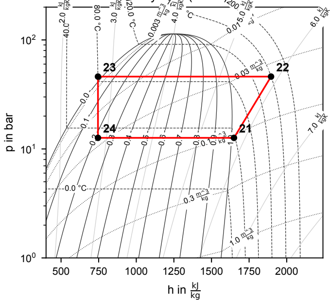
Cycle 1 (R717)
