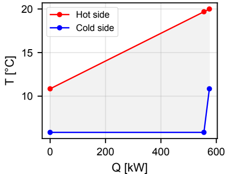
Source HX (cycle-1 evaporator)
