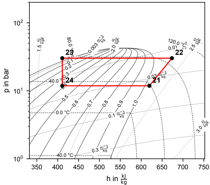
Cycle 1 (R290)
