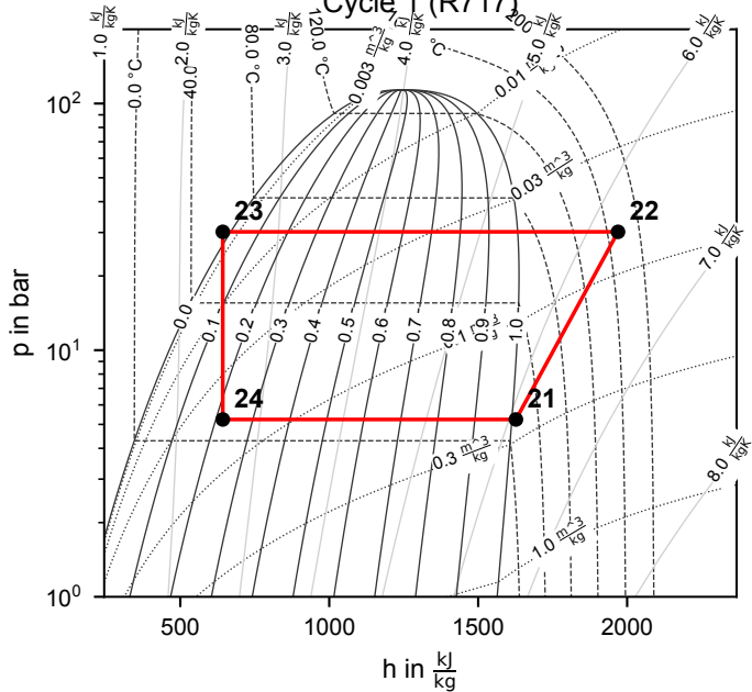
Cycle 1 (R717)
