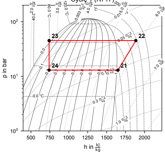
Cycle 1 (R717)
