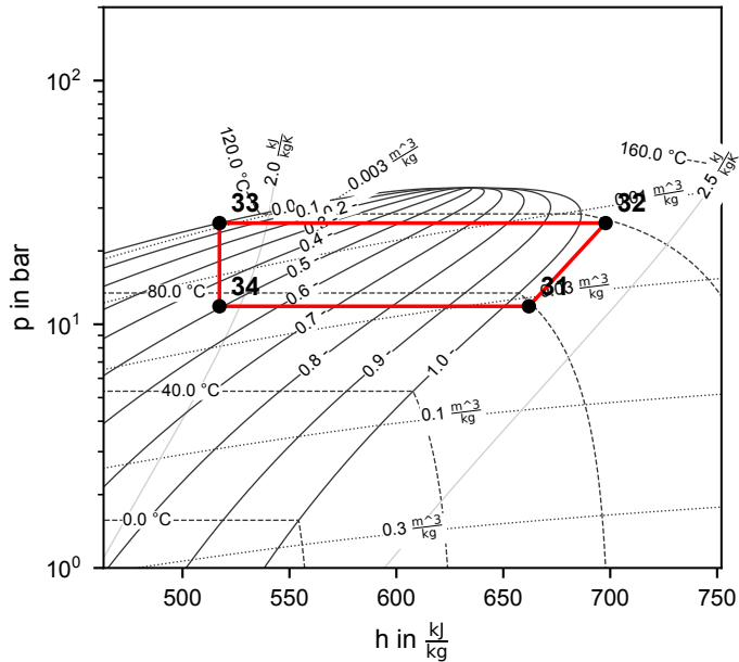
Cycle 2 (R600a)
