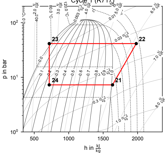
Cycle 1 (R717)
