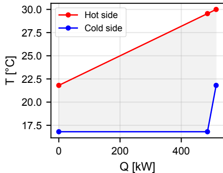
Source HX (cycle-1 evaporator)
