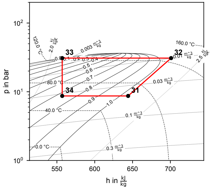
Cycle 2 (R600a)
