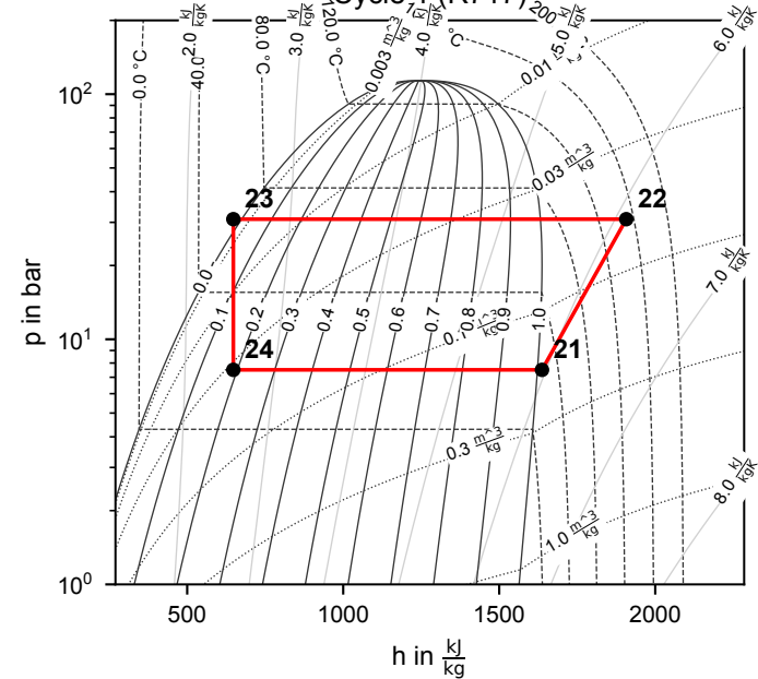
Cycle 1 (R717)
