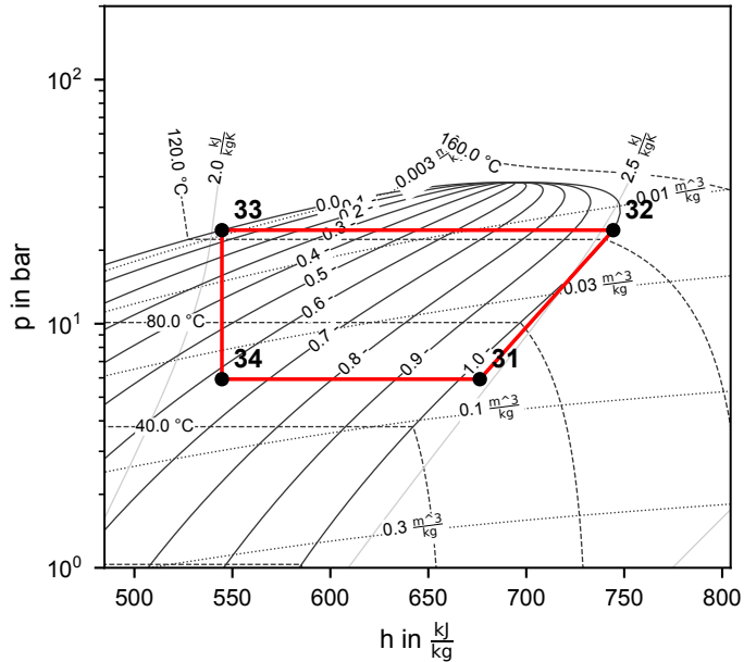
Cycle 2 (R600)
