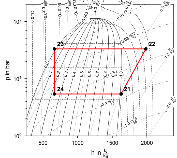
Cycle 1 (R717)
