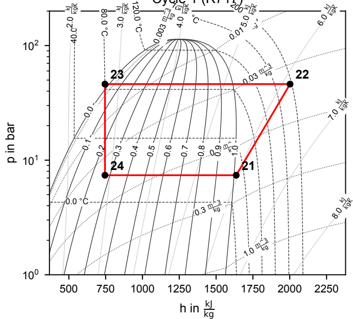
Cycle 1 (R717)
