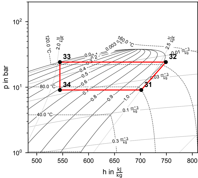
Cycle 2 (R600)
