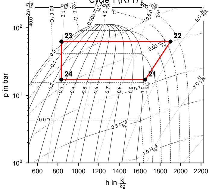
Cycle 1 (R717)
