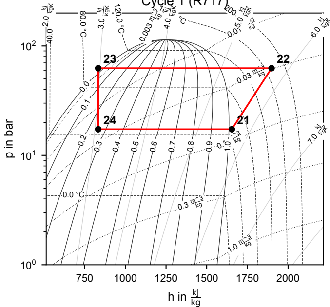
Cycle 1 (R717)
