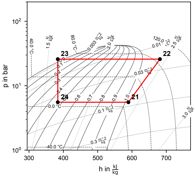
Cycle 1 (R290)
