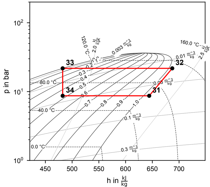
Cycle 2 (R600a)
