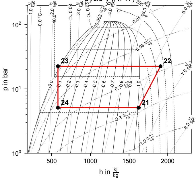
Cycle 1 (R717)
