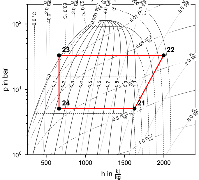
Cycle 1 (R717)
