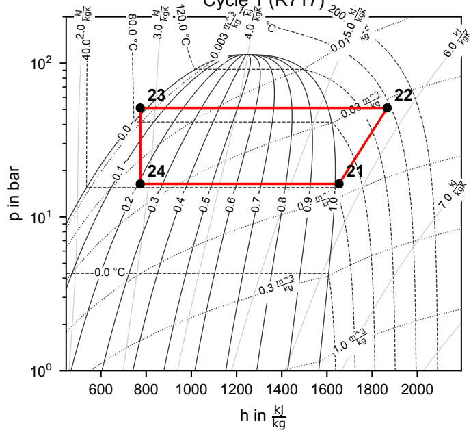
Cycle 1 (R717)
