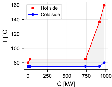
Internal HX (cycle-1 cond. / cycle-2 evap.)
