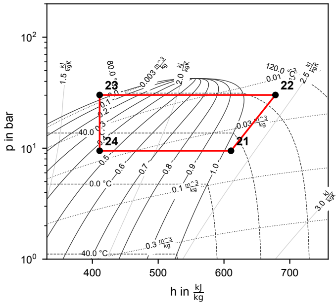
Cycle 1 (R290)
