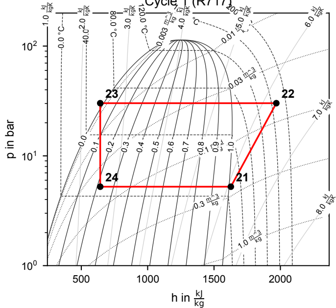
Cycle 1 (R717)
