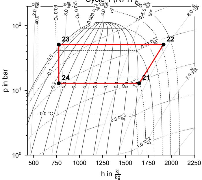
Cycle 1 (R717)
