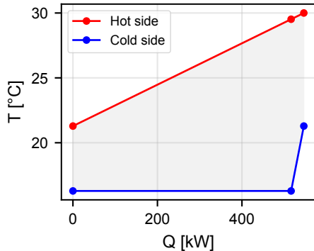
Source HX (cycle-1 evaporator)
