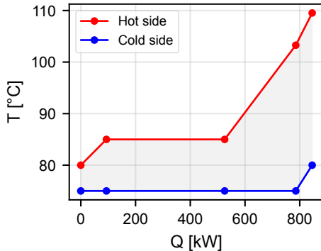
Internal HX (cycle-1 cond. / cycle-2 evap.)
