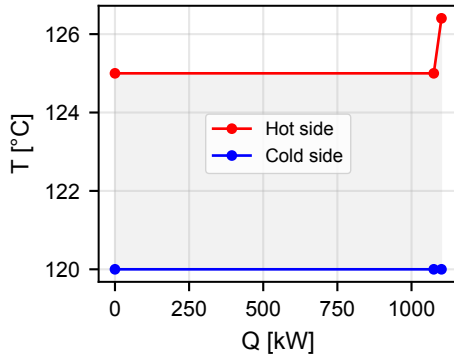
Sink HX (cycle-2 condenser, steam)
