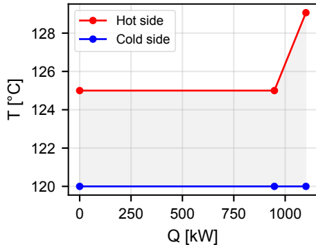
Sink HX (cycle-2 condenser, steam)
