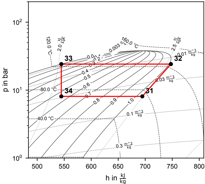
Cycle 2 (R600)
