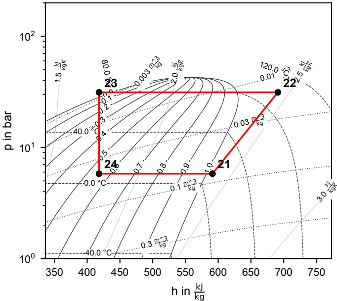
Cycle 1 (R290)
