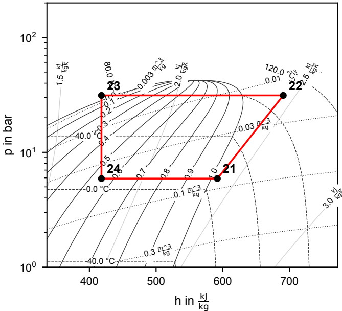
Cycle 1 (R290)
