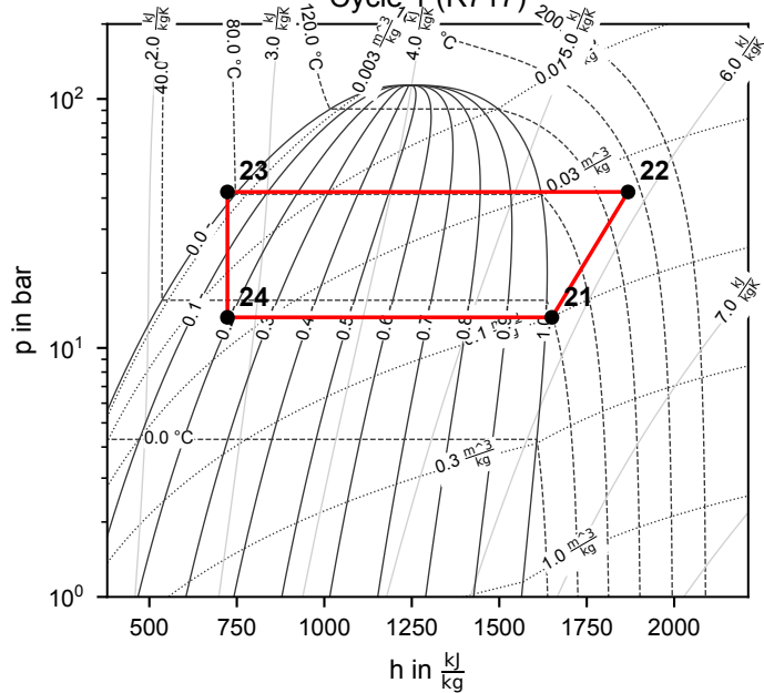
Cycle 1 (R717)
