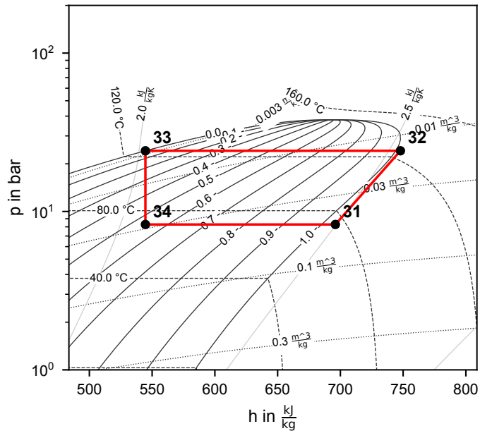
Cycle 2 (R600)
