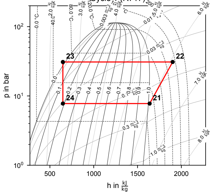
Cycle 1 (R717)
