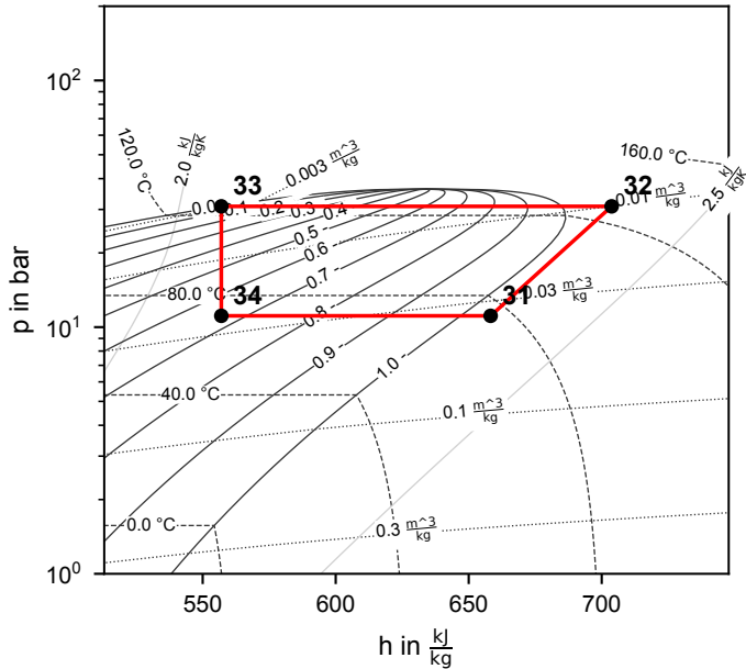
Cycle 2 (R600a)
