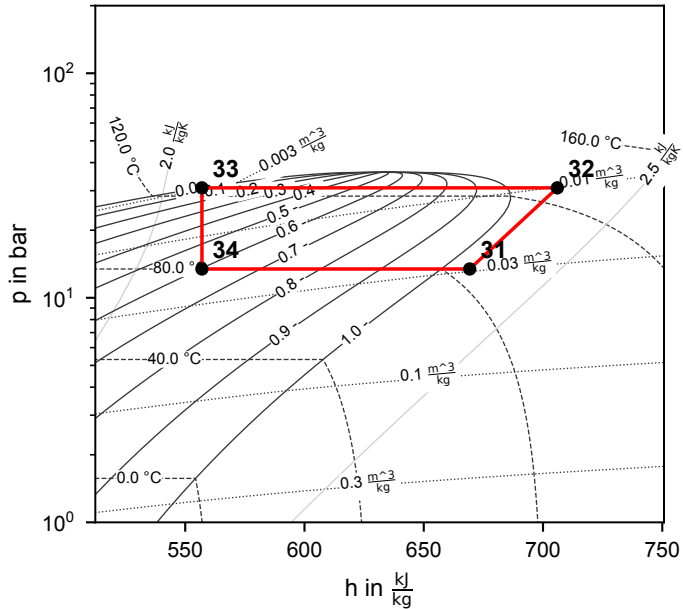
Cycle 2 (R600a)
