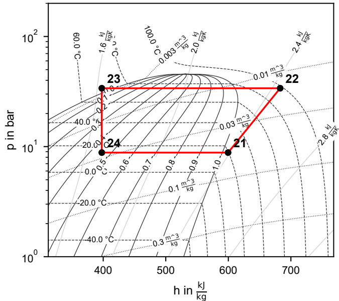
Cycle 1 (R1270)
