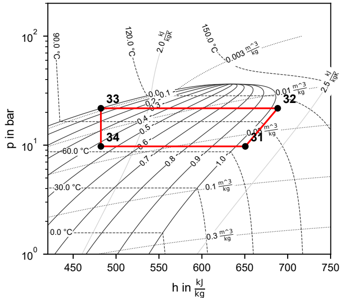
Cycle 2 (R600a)
