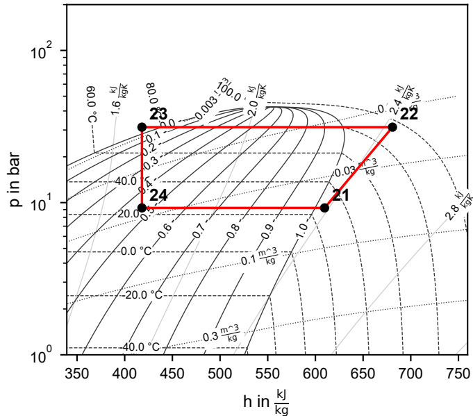
Cycle 1 (R290)
