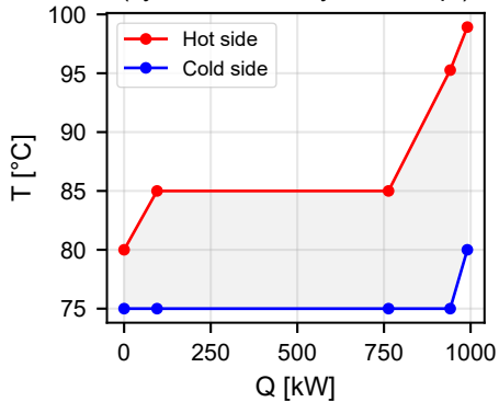
Internal HX (cycle-1 cond. / cycle-2 evap.)
