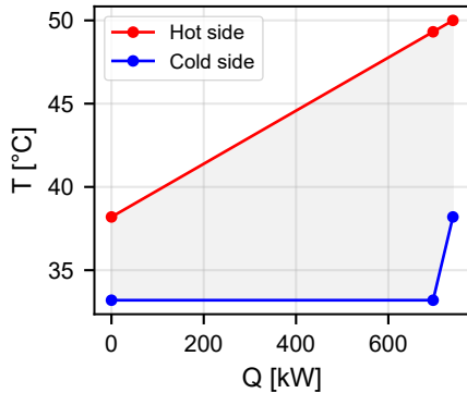
Source HX (cycle-1 evaporator)
