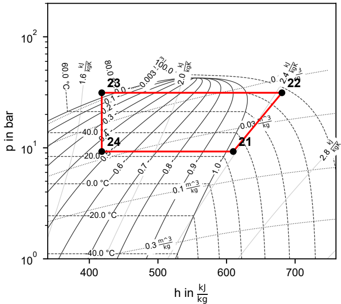
Cycle 1 (R290)
