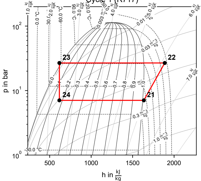
Cycle 1 (R717)
