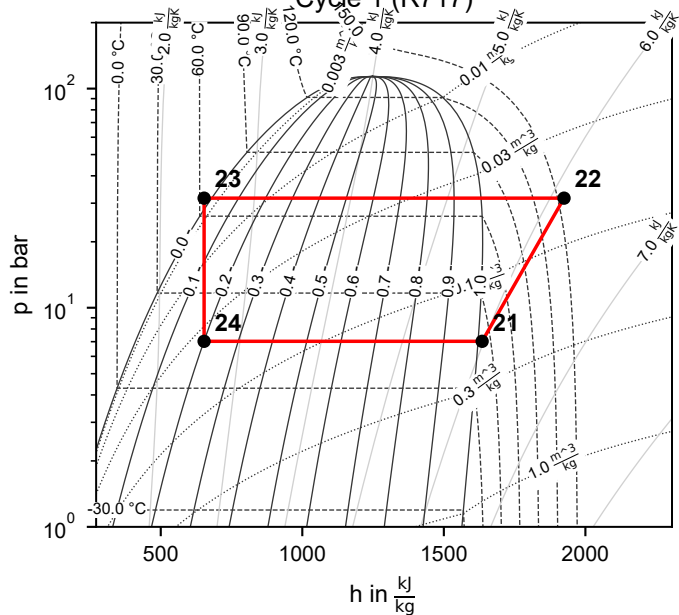
Cycle 1 (R717)
