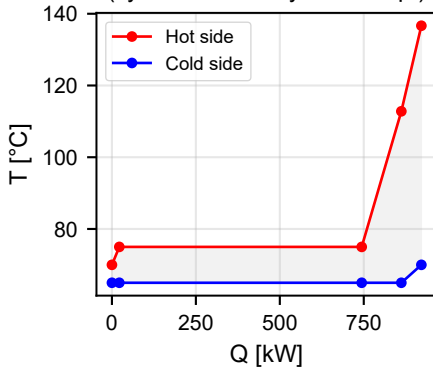
Internal HX (cycle-1 cond. / cycle-2 evap.)
