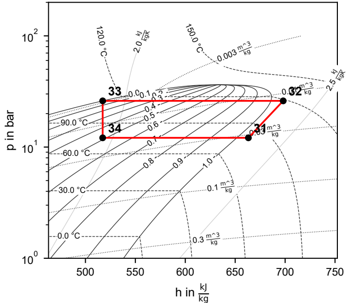
Cycle 2 (R600a)
