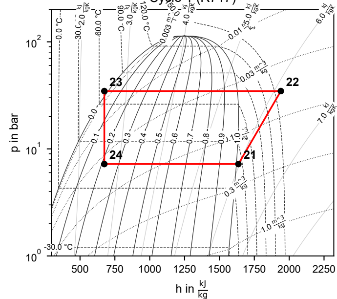
Cycle 1 (R717)
