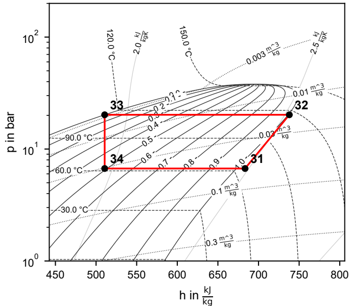
Cycle 2 (R600)
