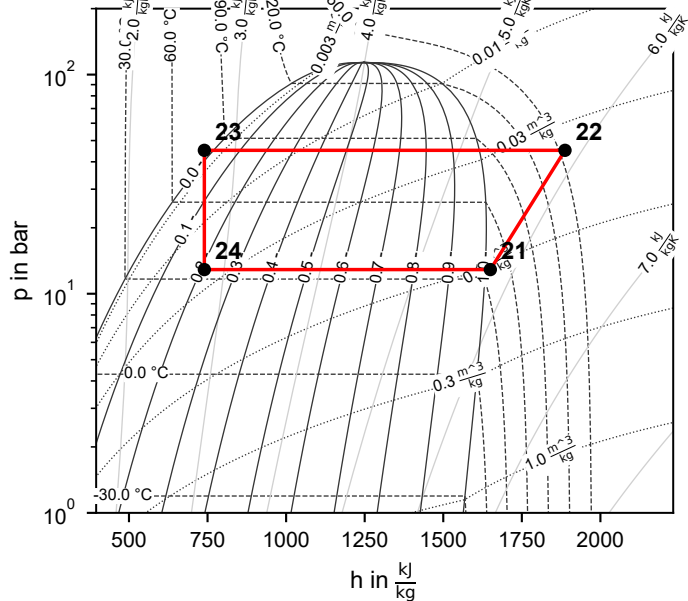
Cycle 1 (R717)
