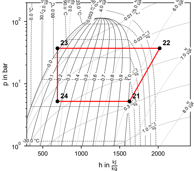
Cycle 1 (R717)
