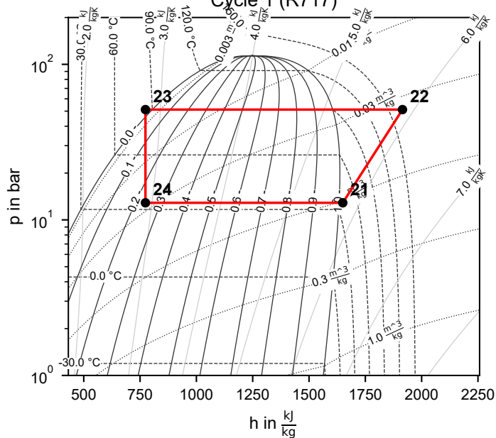
Cycle 1 (R717)
