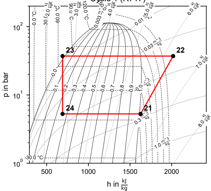
Cycle 1 (R717)
