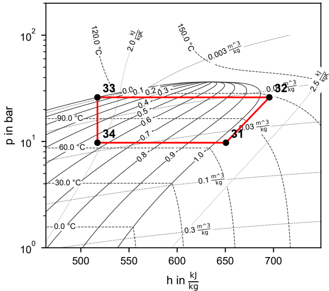
Cycle 2 (R600a)
